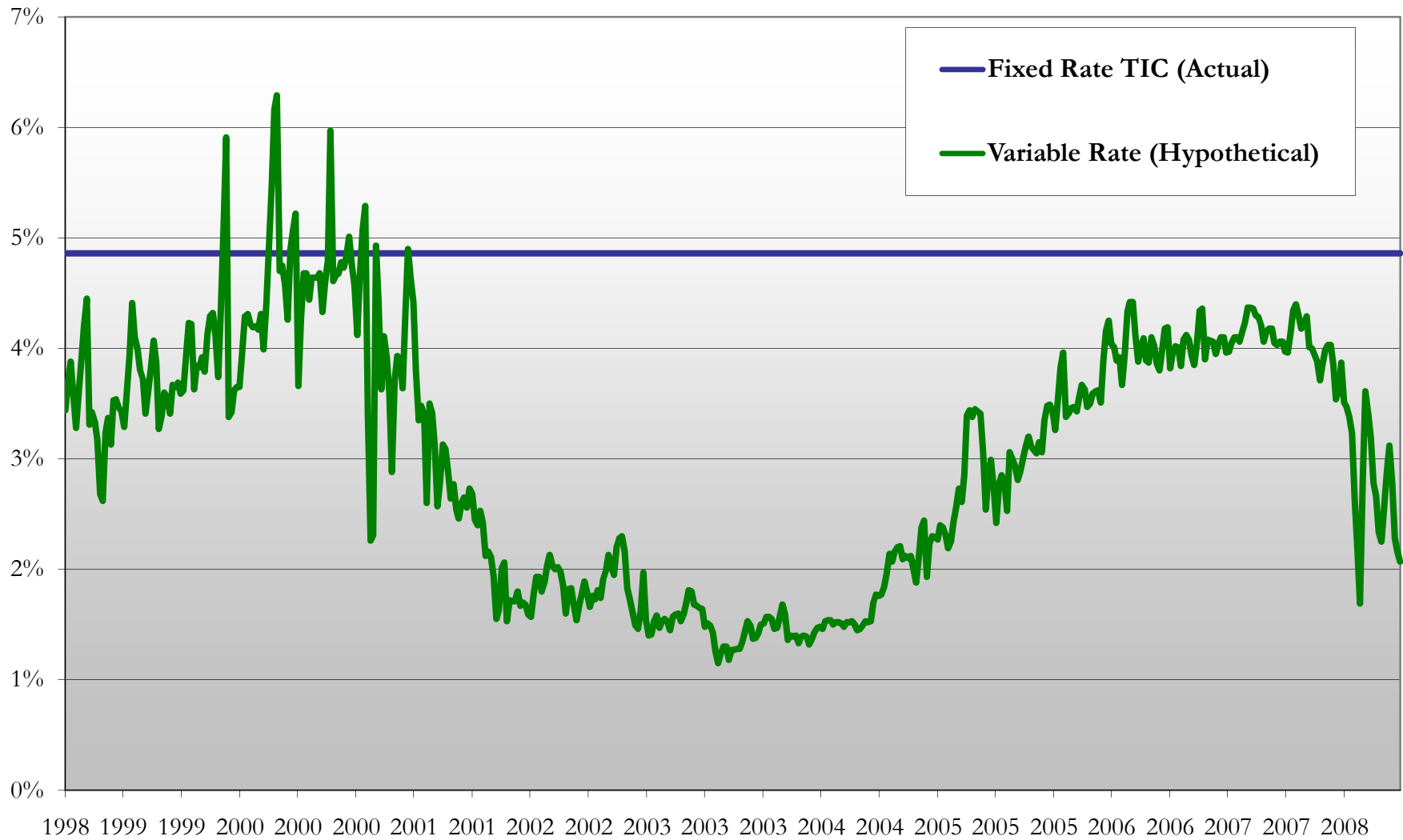
Series 1998DE: Actual and Hypothetical Interest Rates From 11/1/1998 to 5/30/2008
